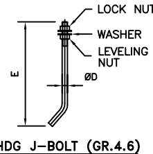
HDG J-BOLT (GR.4.6)
