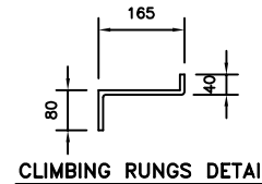
CLIMBING RUNGS DETAIL
