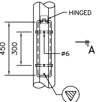
SERVICE DOOR DETAIL
