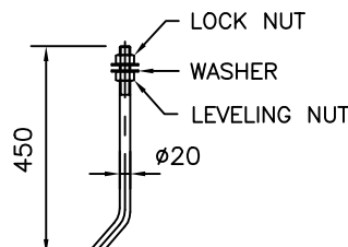
J-BOLT
