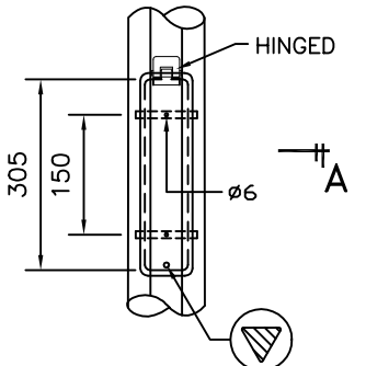
STAINLESS STEEL LOCKING BOLT
