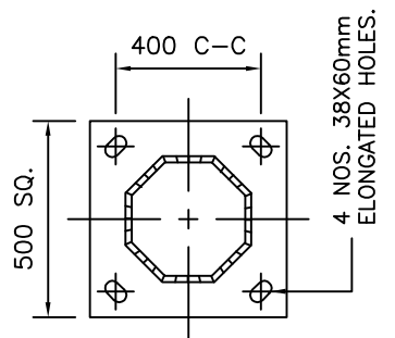
SECTION X-X
