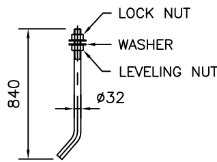
J-BOLT
